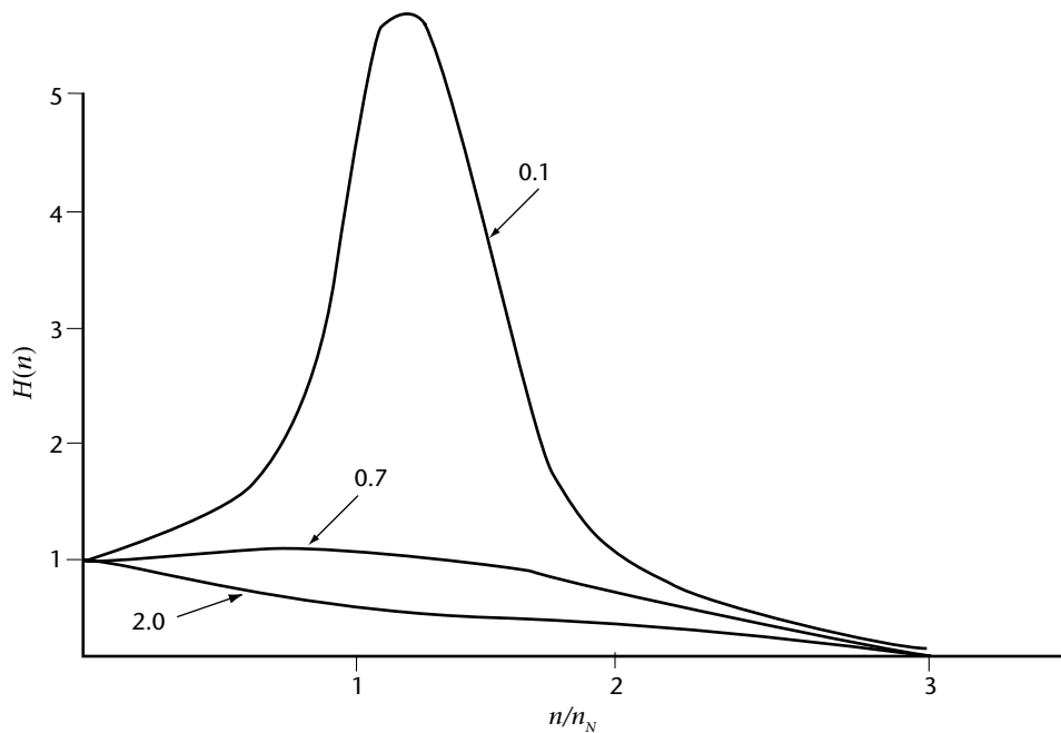
Figure 2.7. Frequency response functions for a second order system, such as a wind vane. The frequency is normalized by n_N the natural frequency, which depends on wind speed. The curves shown are for damping factors with values 0.1 (very lightly damped), 0.7 (critically damped, optimum for most purposes) and 2.0 (heavily damped).
