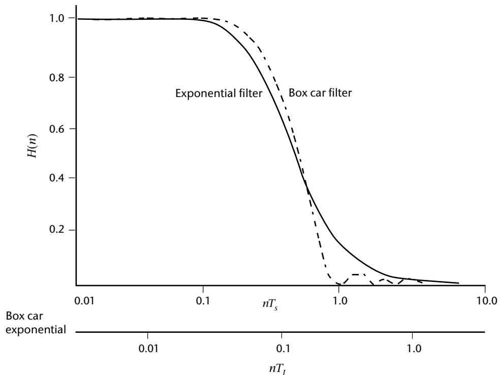
Figure 2.6. Frequency response functions for a first order (exponential) weighting function and a box car weighting function. The frequency is normalized for the first order filter by T_I , the time constant, and for the box car filter by T_s , the sampling time.
